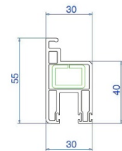
Hoja mosquitero 100SN5730
