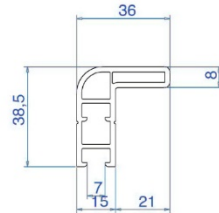
Riel mosquitero 100SN5720
